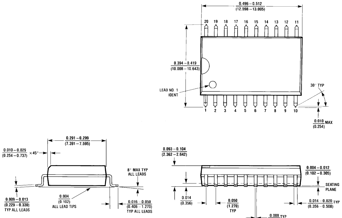
Wide-Body Small-Outline Package (M) Order Number ADC08061CIWM, or ADC08062CIWM NS Package Number M20B
